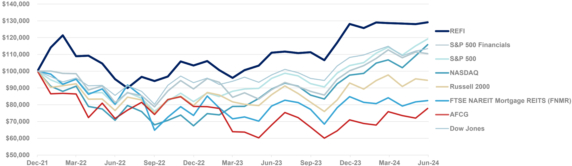
Illustrative Quarterly Growth of $100,000 Invested, from Dec 31, 2021 to June 30, 2024
